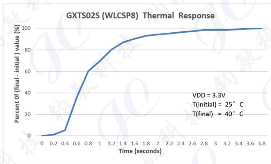
Figure3 Thermal Response of the GXTS02S sensor.
